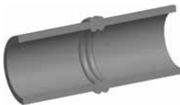
Figure C.3: Bead design at heated tool butt welding (principle) of a pipe.
