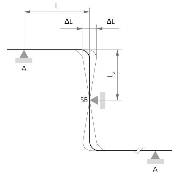
Figure B.4: Z-compensation.
